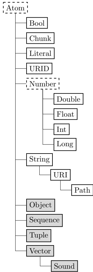
Figure 1: The Atom type hierarchy. Abstract types are dashed, and collections are grey.
